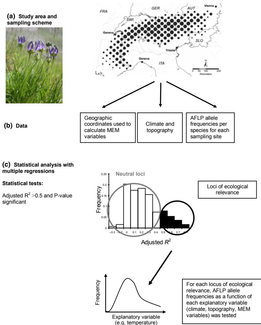
Fig. 1 Approach used in this study to detect loci of ecological relevance in 13 alpine plant species. (a) Map of the European Alps showing the study range and sampling intensity (circle area proportional to number of species genotyped per grid cell). (AUT, Austria; FRA, France; GER, Germany; ITA, Italy; SLO, Slovenia; SWI, Switzerland). The number of sampling sites per species is given in Table 1. (b) Type of genetic, environmental and spatial data (MEM variables: Moran’s eigenvector maps) used. (c) Schematic of the statistical analyses. The example given in (a) is Phyteuma hemisphaericum , one of the alpine plants studied.
