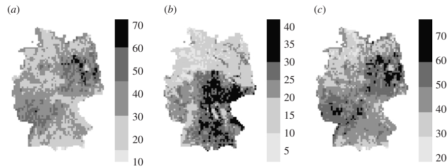
Figure 1. Percentages of species (a) loss, (b) gain and (c) turnover from GLM ( 6' \times 10' ) for the GRAS scenario for Germany. Modelled estimates of loss, gain, turnover across models (GLM, GAM and RF) showed high agreement (table S2 in the electronic supplementary material).
